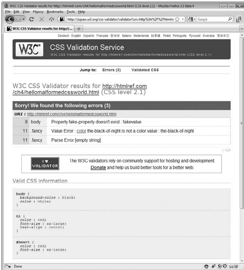
FIGURE 4-6 Validating CSS
