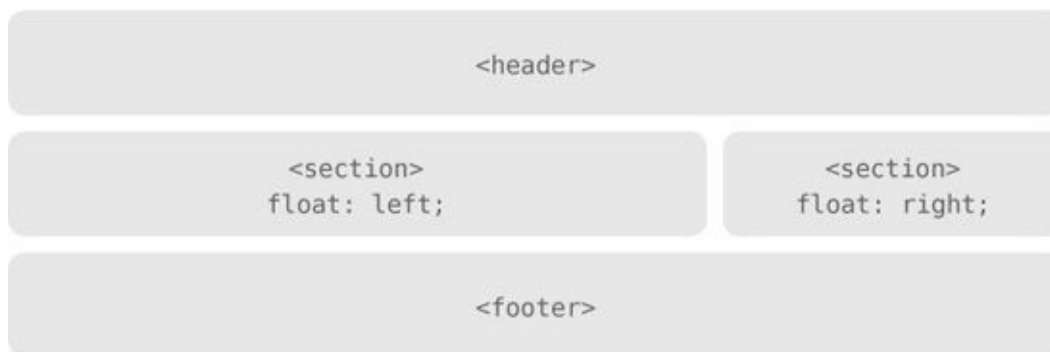
Figure 5.2 A two-column page layout using floats
