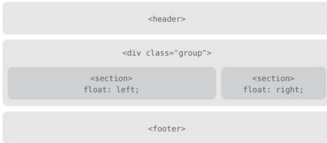
Figure 5.6 A two-column page layout with contained floats
