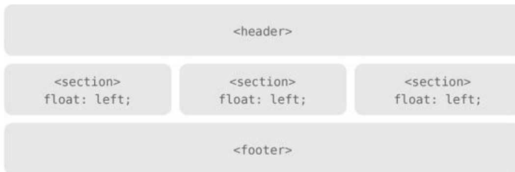
Figure 5.3 A three-column page layout using floats
