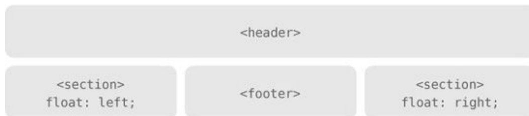
Figure 5.4 A two-column page layout without any identified column widths or cleared floats
